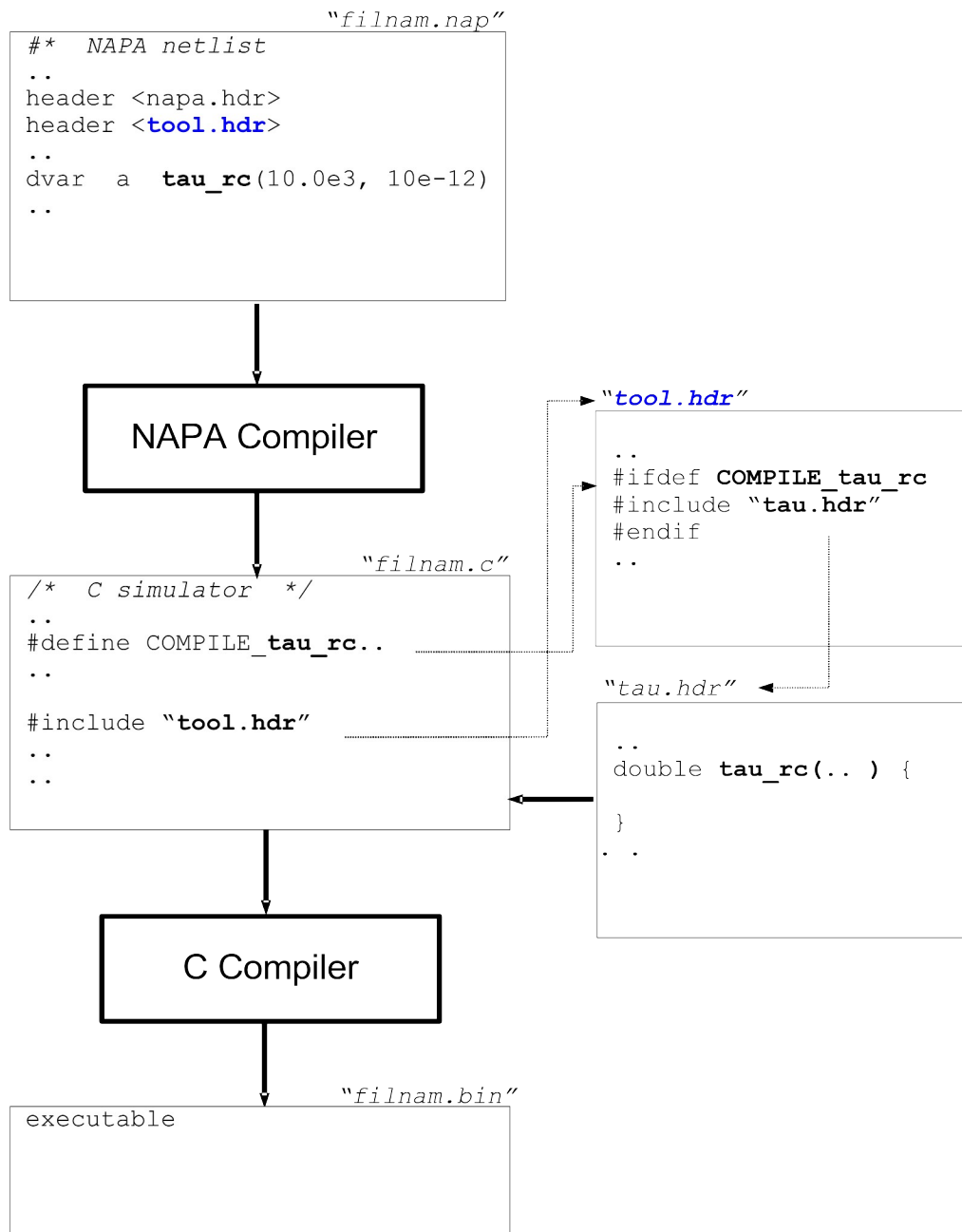
Figure 17 - The C macroprocessor and the functions
