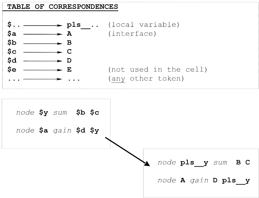
Figure 9 - The parsing mechanism of a cell (b)
