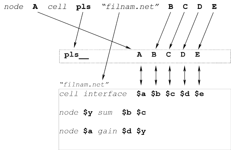
Figure 8 - The parsing mechanism of a cell (a)
