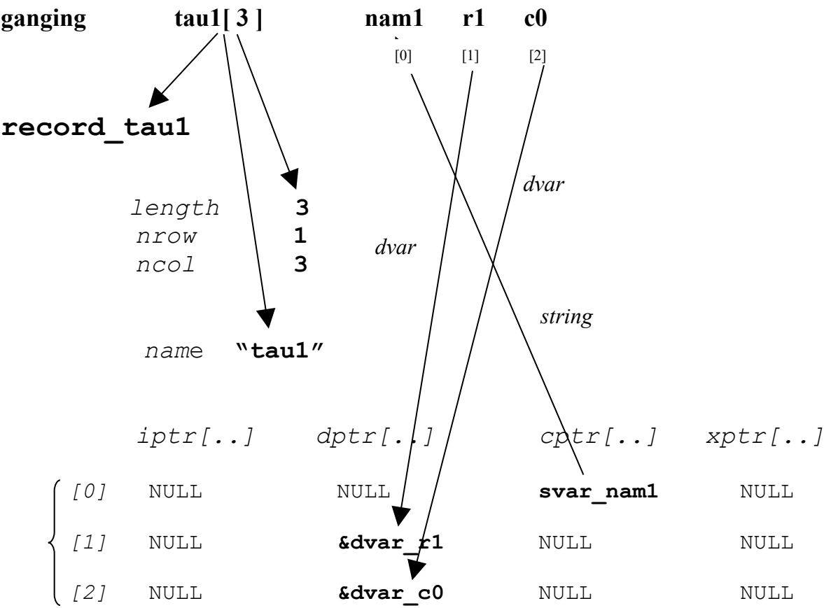
Figure 23 - How NAPA variables are passed by addresses
