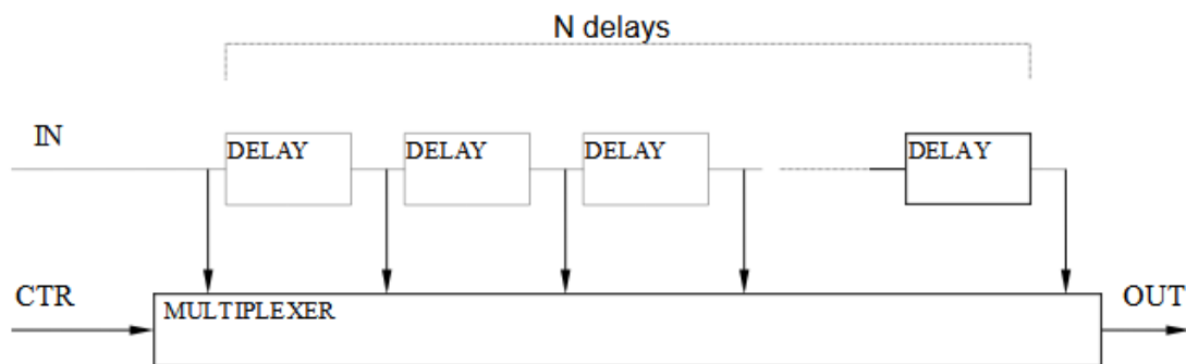
Figure 15 - Programmable delays
