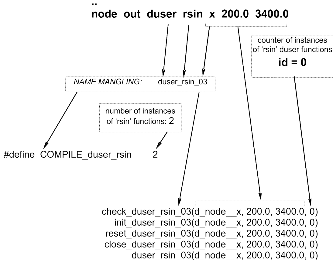
Figure 20 - Name mangling for a user-defined function "duser"
